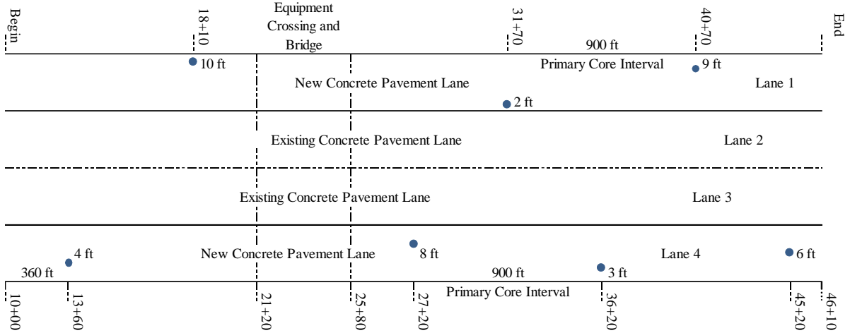
Figure 4-40.1. Primary Cores
