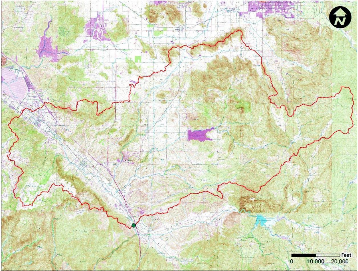
Figure B3.4. Threshold drainage area, Example 3.
