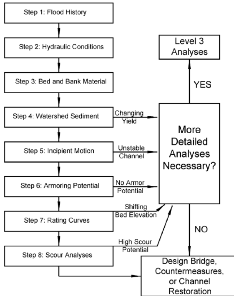
Figure B2.11. Flow chart for Level 2: Basic Engineering Analysis. From Lagasse et al. (2012)
