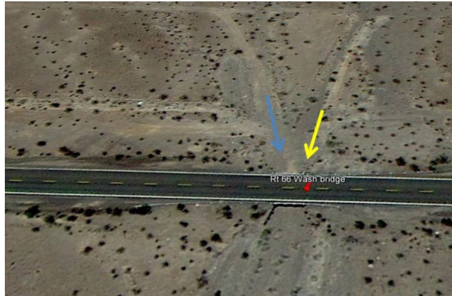
Figure B2.10. Stream crossing alignment with upstream flow in main channel (yellow arrow) complicated by tributary gully (blue arrow), unnamed wash 3.5 miles east of Ludlow, California. Looking upstream.
