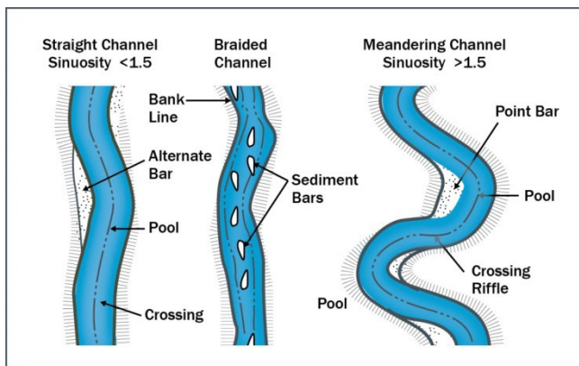
Figure 14. Plan View of Major Channel Patterns
