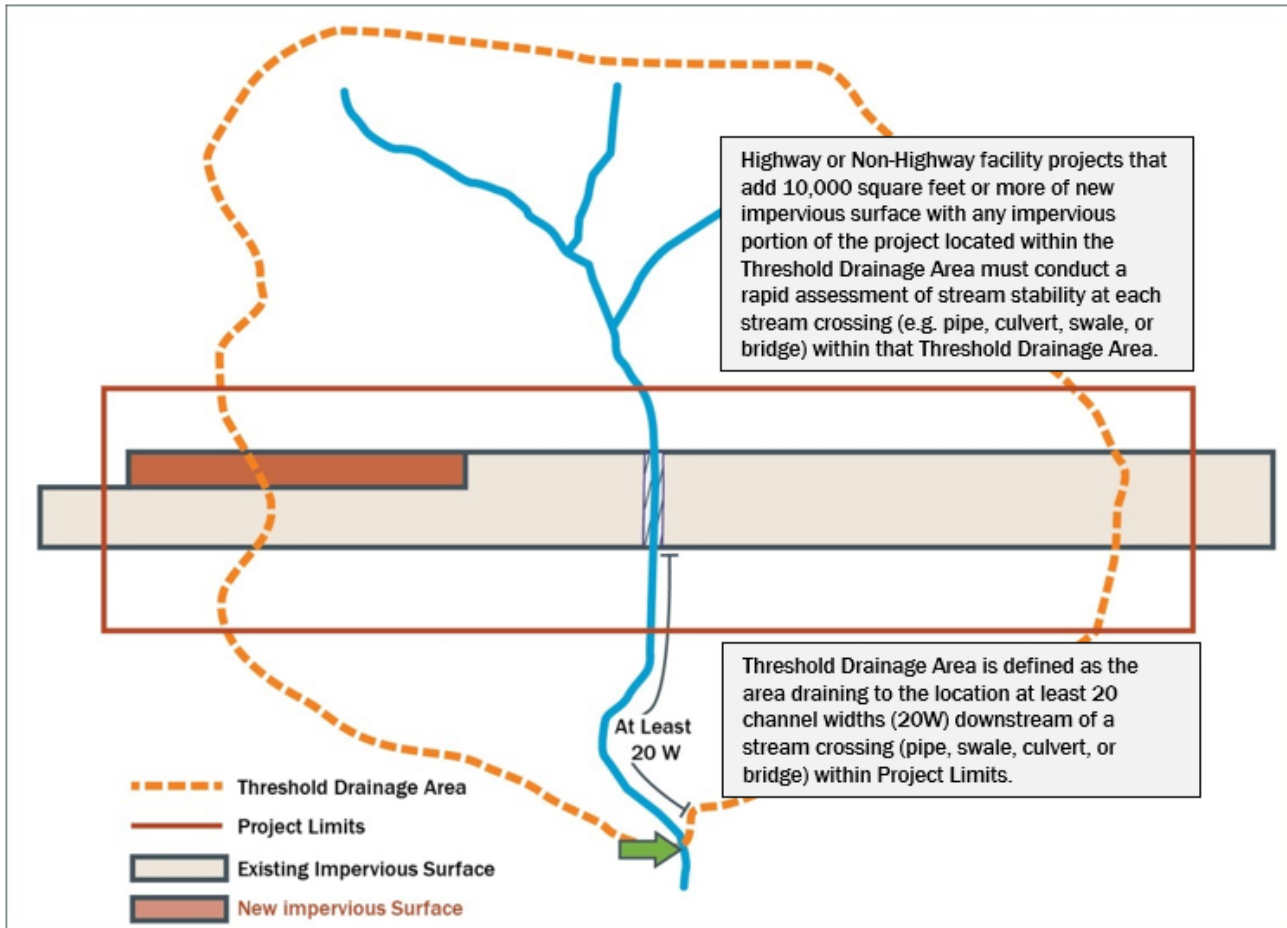
Figure 1. Definition of Threshold Drainage Area (TDA)
