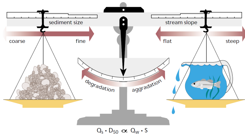
Figure 5. Schematic Illustrating Lane’s Relation
