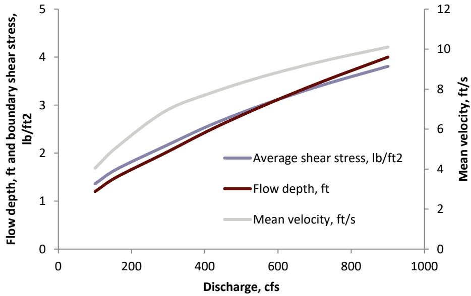
Figure B2.12. Hydraulic characteristics of representative reach, Route 66 Wash near Ludlow, based on assumption of uniform flow.
