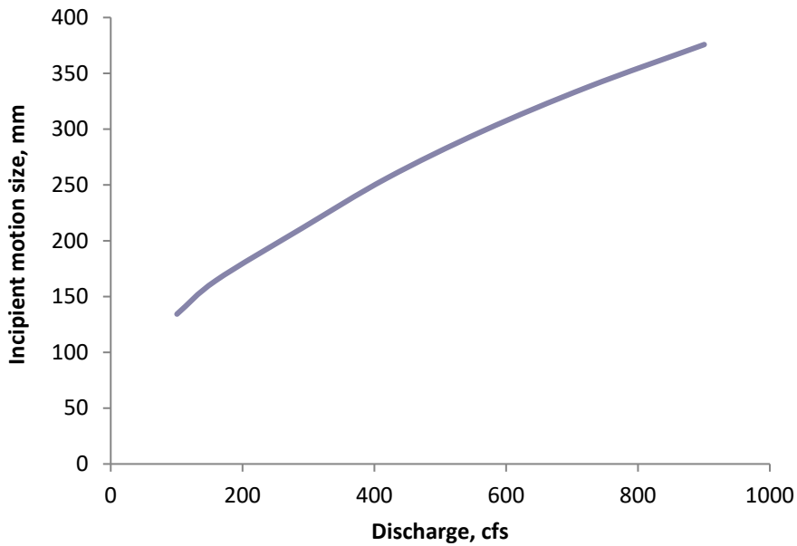
Figure B2.13. Incipient motion size for representative reach, Route 66 Wash near Ludlow.
