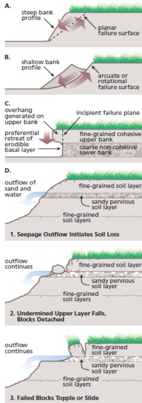
Figure 6. Common Mechanisms for Mass Failure of Streambanks
