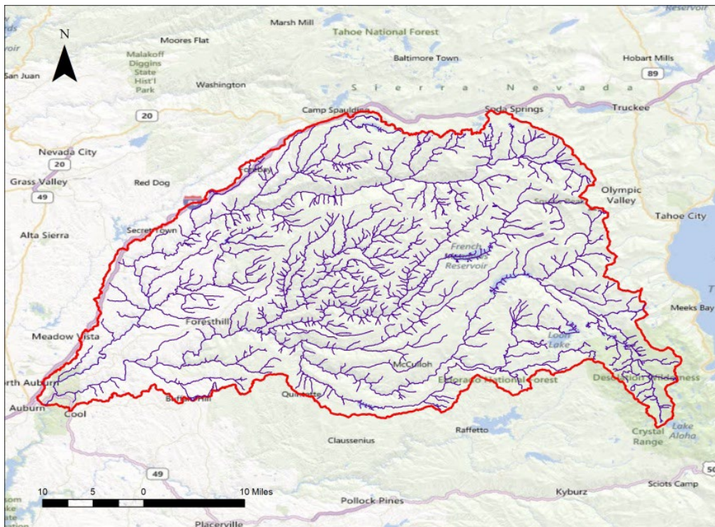
Figure B1.4. Threshold drainage area, Example 1.
