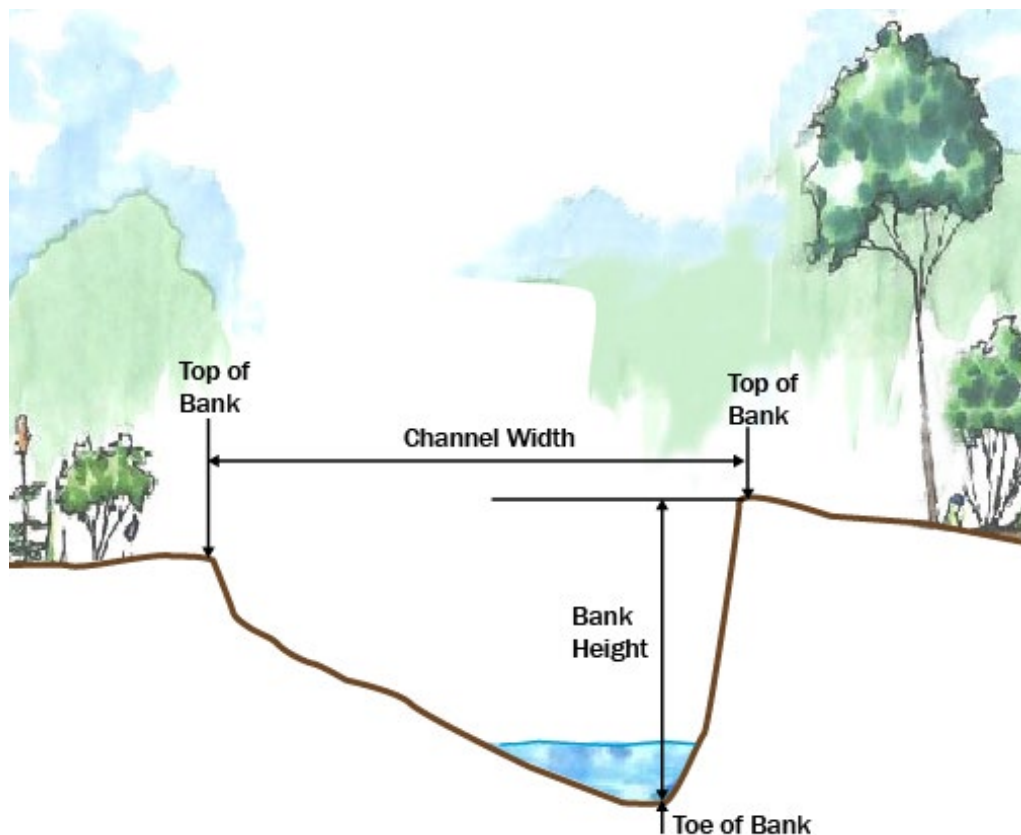
Figure 2. Definition of Top Bank and Other Channel Features
