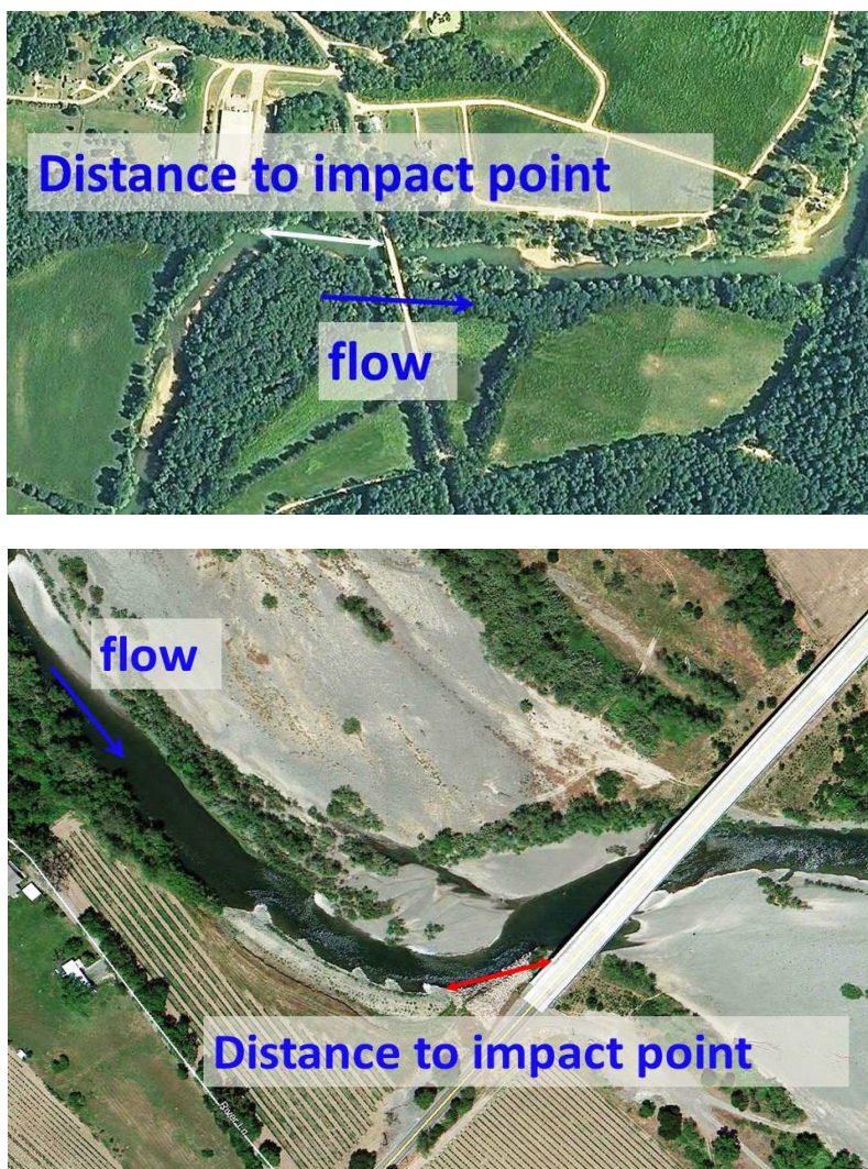
Figure 25. Stream Crossing Alignment with Flow Examples
