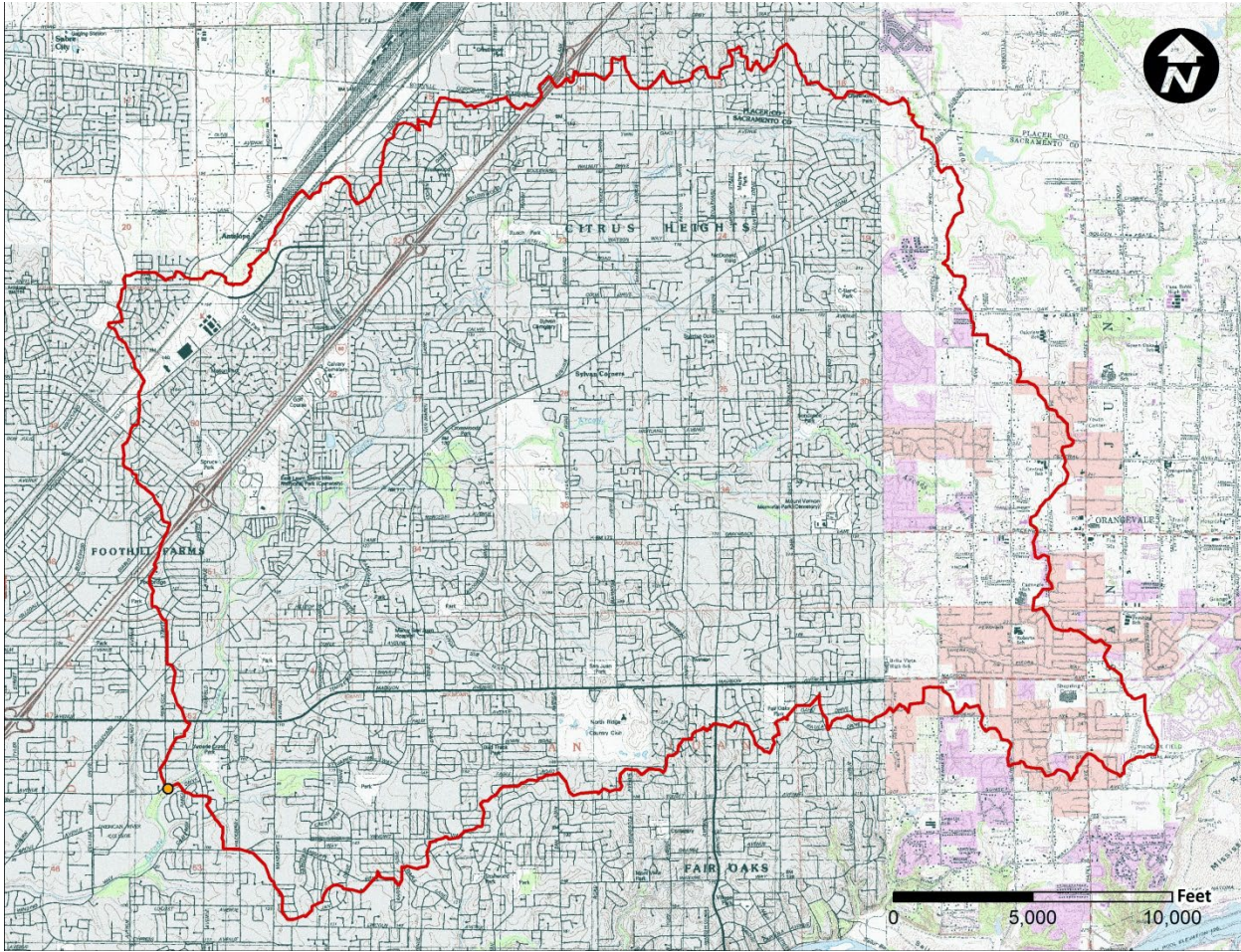
Figure B4.4. Threshold drainage area, Example 4.
