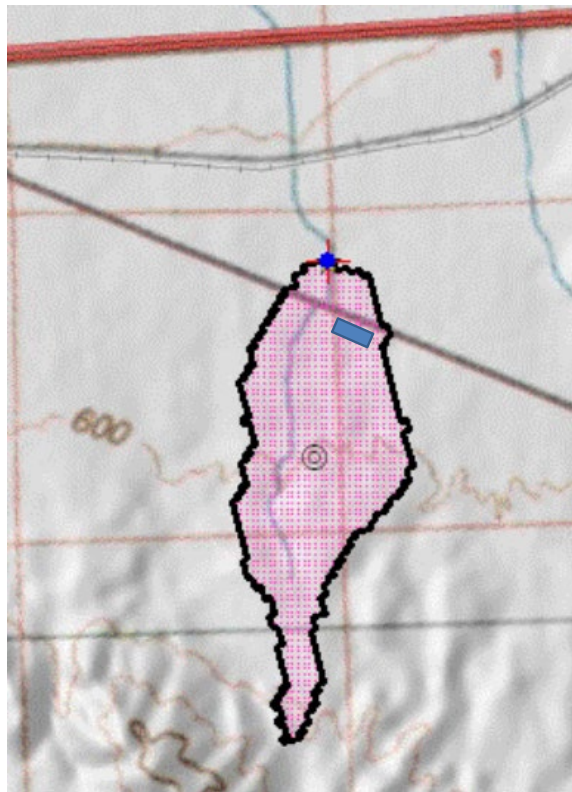
Figure B2.4. Threshold drainage area, Example 2. Gray rectangle indicates new impervious area.
