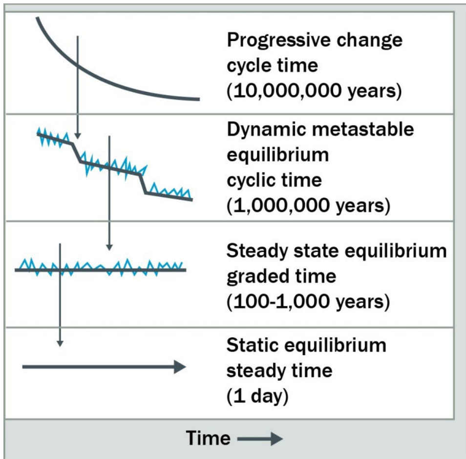
Figure 4. Time Scales in Geomorphic Systems
