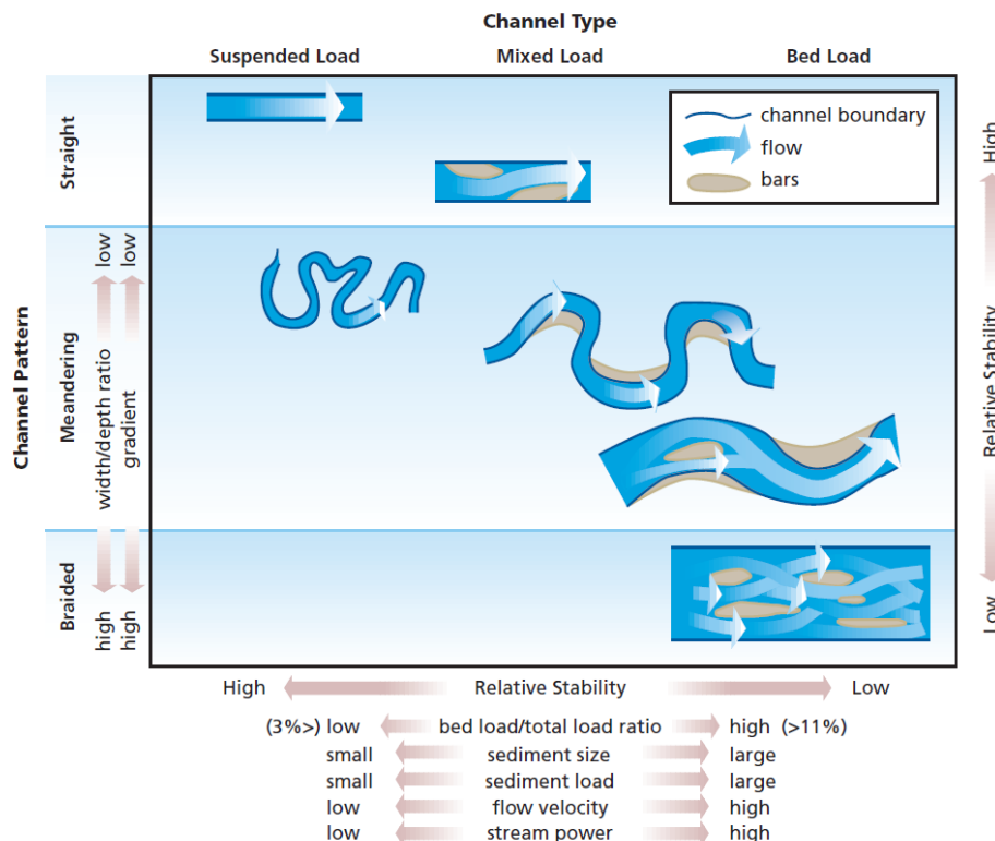
Figure 10. Simple Stream Classification System
