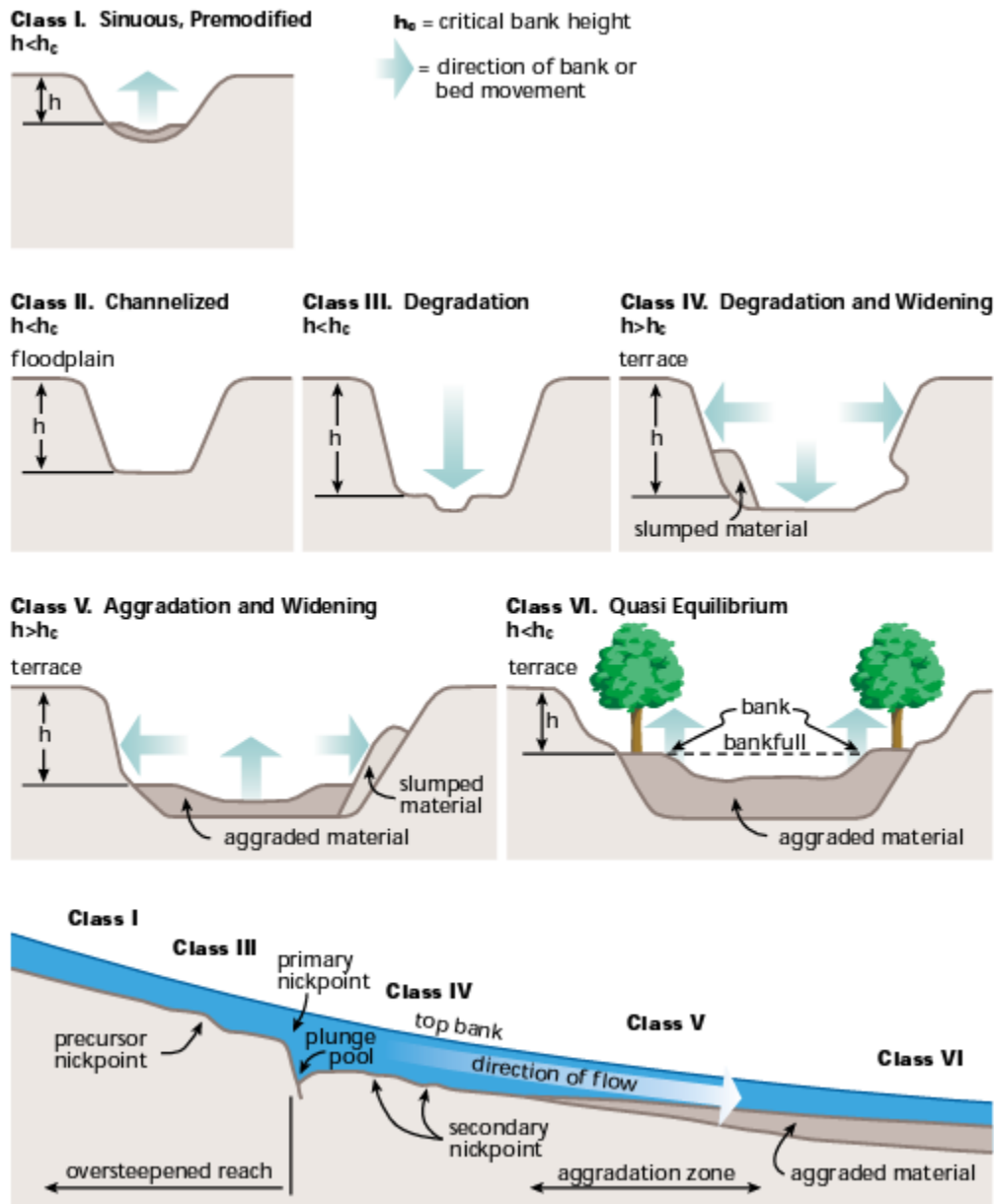
Figure 7. Schematic of Conceptual Channel Evolution Model (FISRWG 1998)
