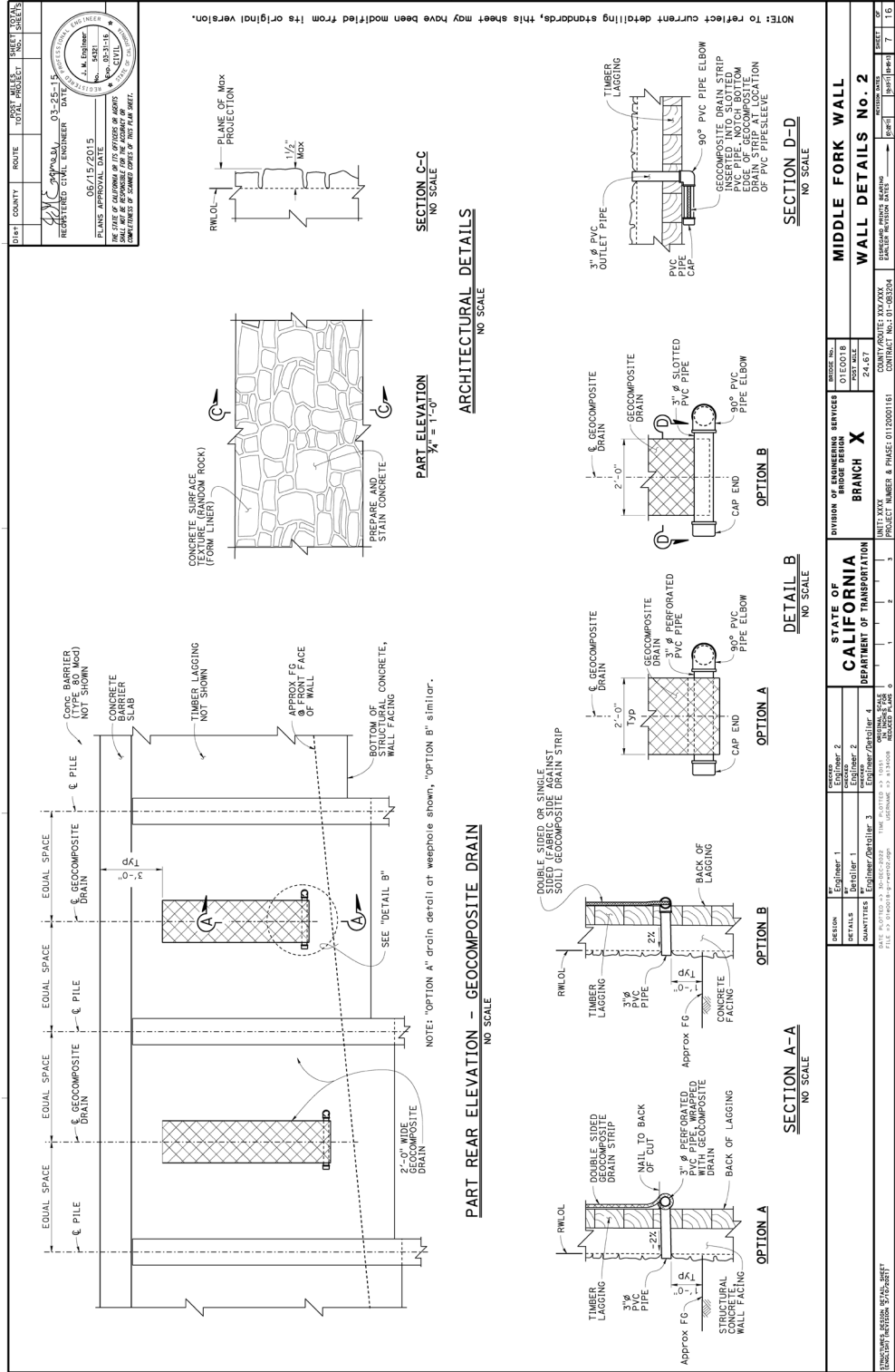
Figure 8A.B.5 Soldier Pile Retaining Wall Detailing Example 5
