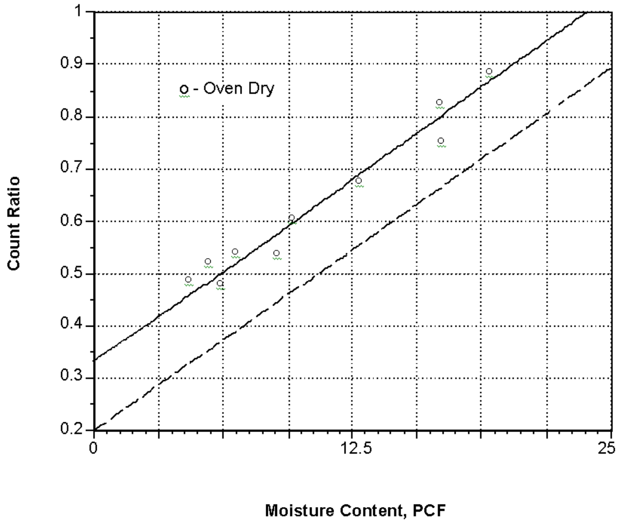
Moisture Calibration Curve
