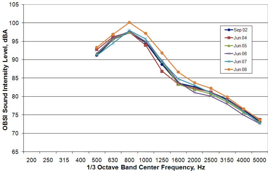
Figure 3-16: 1/3 Octave band OBSI levels during Summer Monitoring Periods, Westbound
