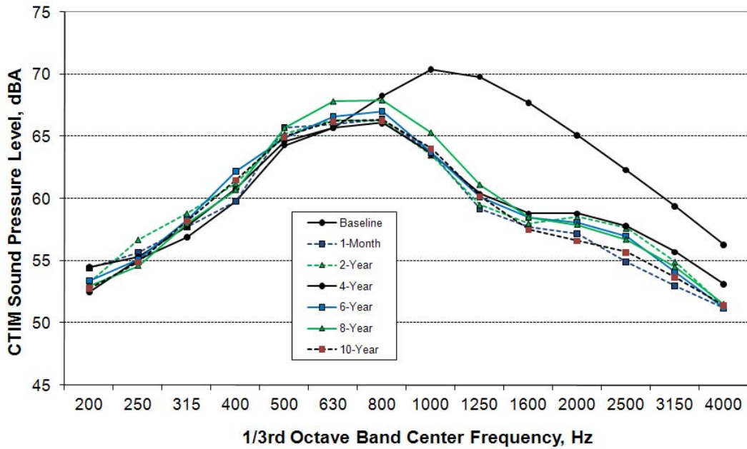
Figure 3-16: 1/3 Octave band OBSI levels during Summer Monitoring Periods, Westbound
