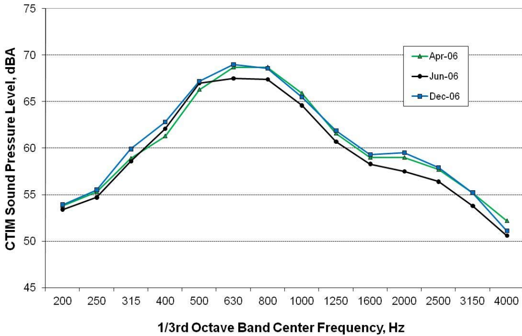
Figure 3-19: 1/3 Octave band levels for OGAC Overlay, 2006 Westbound CTIM Reference
