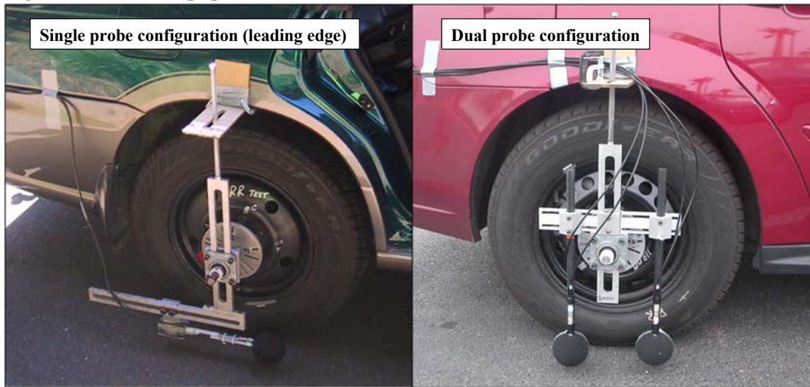
Figure 2-5: Goodyear Aquatred 3 Test Tire
