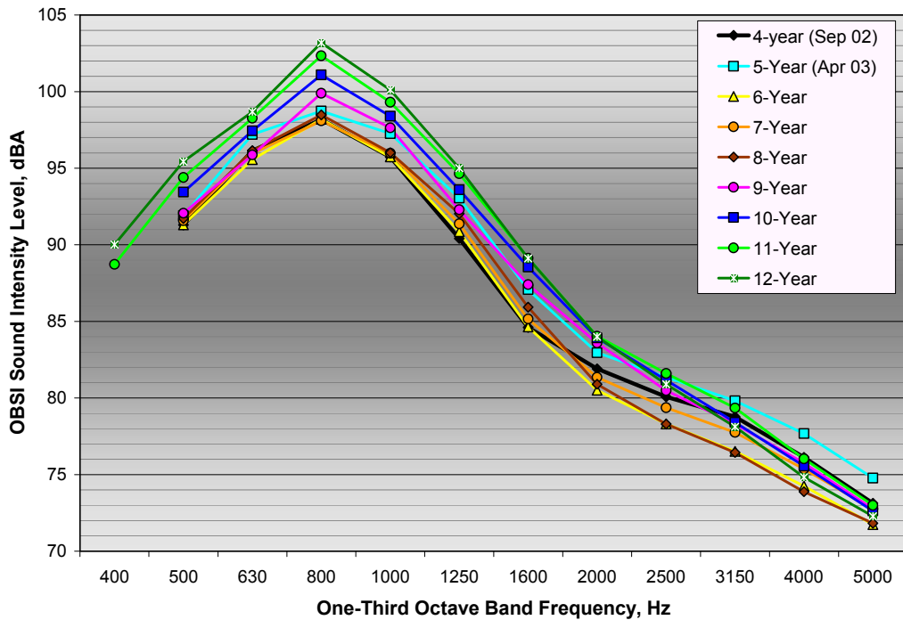
Figure 4-14: One-Third Octave Band OBSI Levels for the Yearly Measurement Periods in the Eastbound Direction
