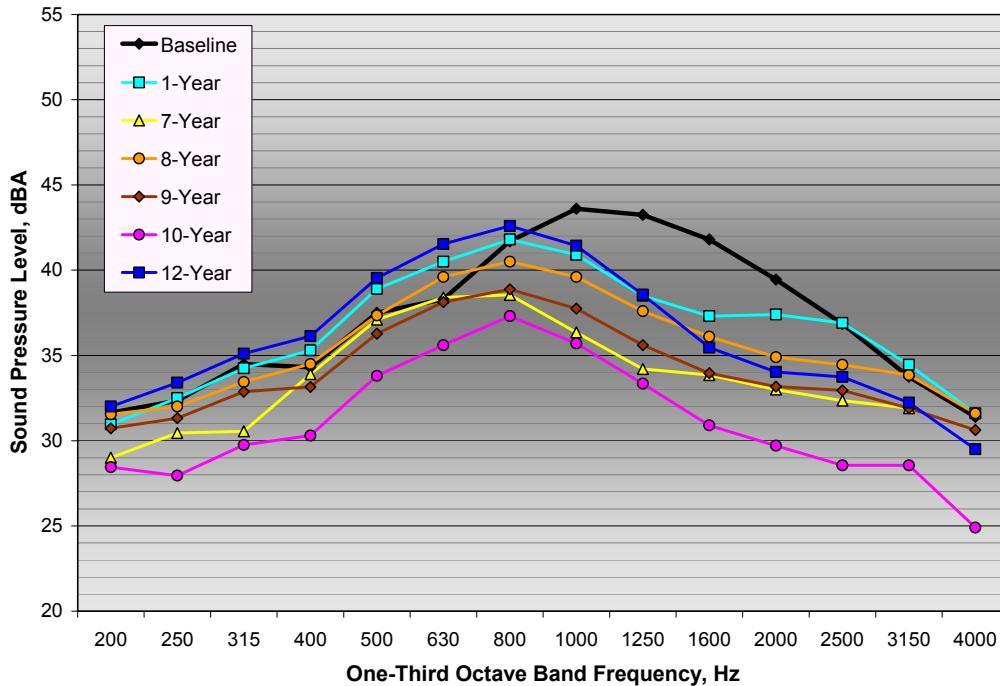
Figure 4-8: One-Third Octave Band Levels for the Yearly Summer Measurement Periods, as well as October 2010, at the Westbound Distant Ground Position Under Upwind Conditions
