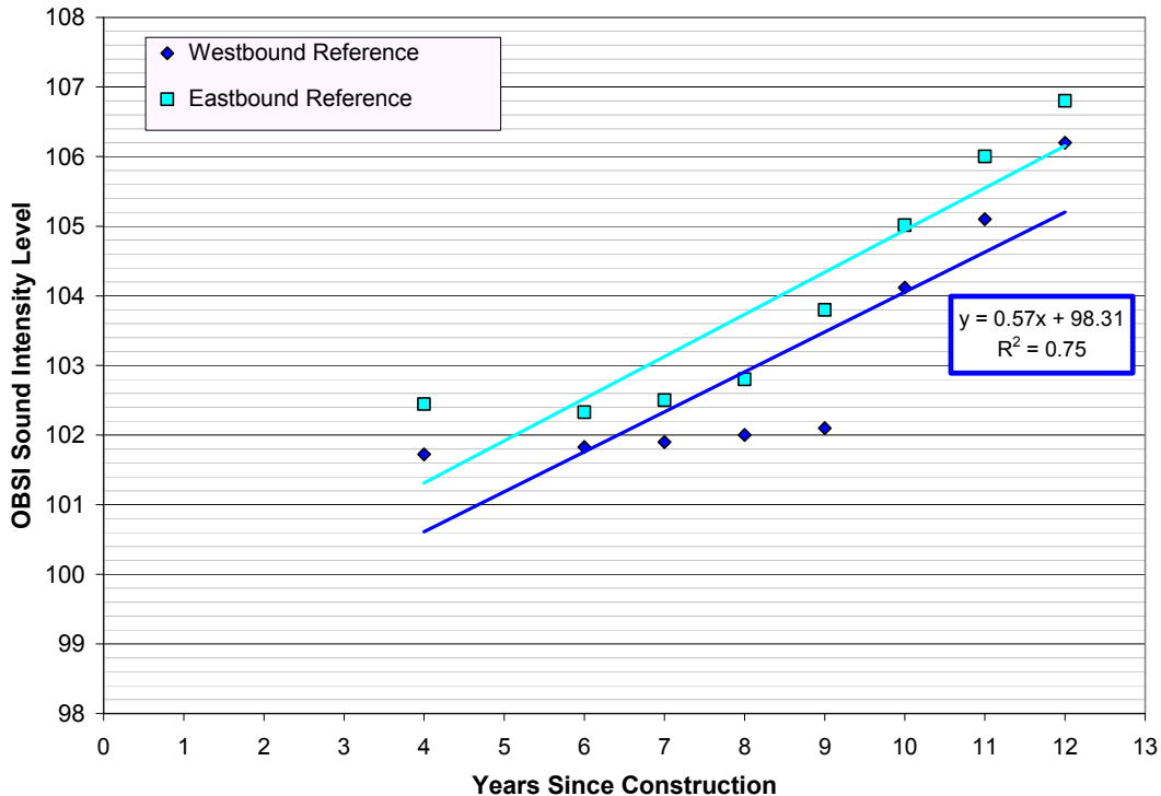
Figure 4-21: Overall OBSI Levels Versus Year of Construction for Outside Lanes of Travel
