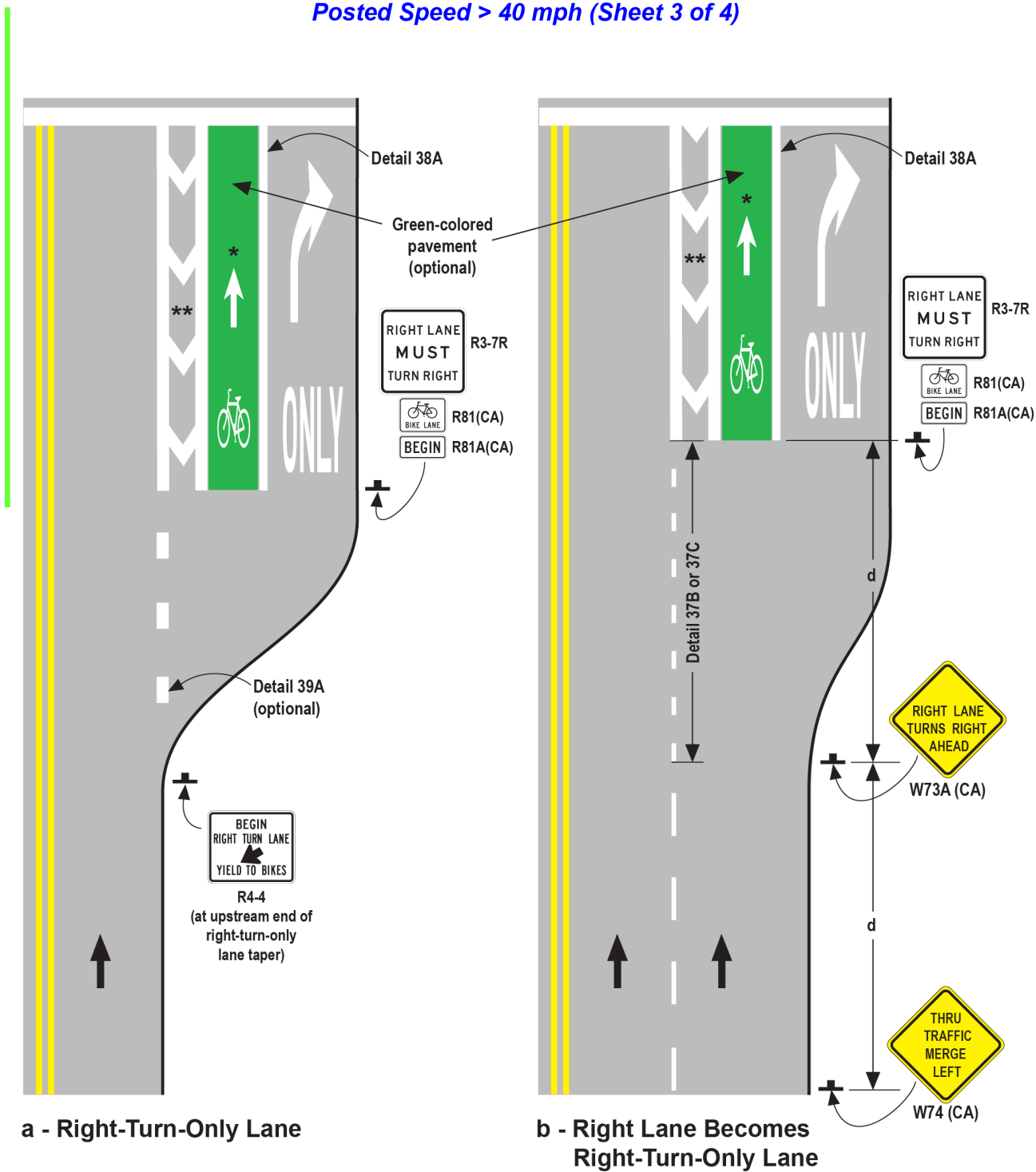
Figure 9C-4 (CA). Example of Bicycle Lane Treatment at a Right Turn Only Lane, Posted Speed > 40 mph (Sheet 3 of 4)
