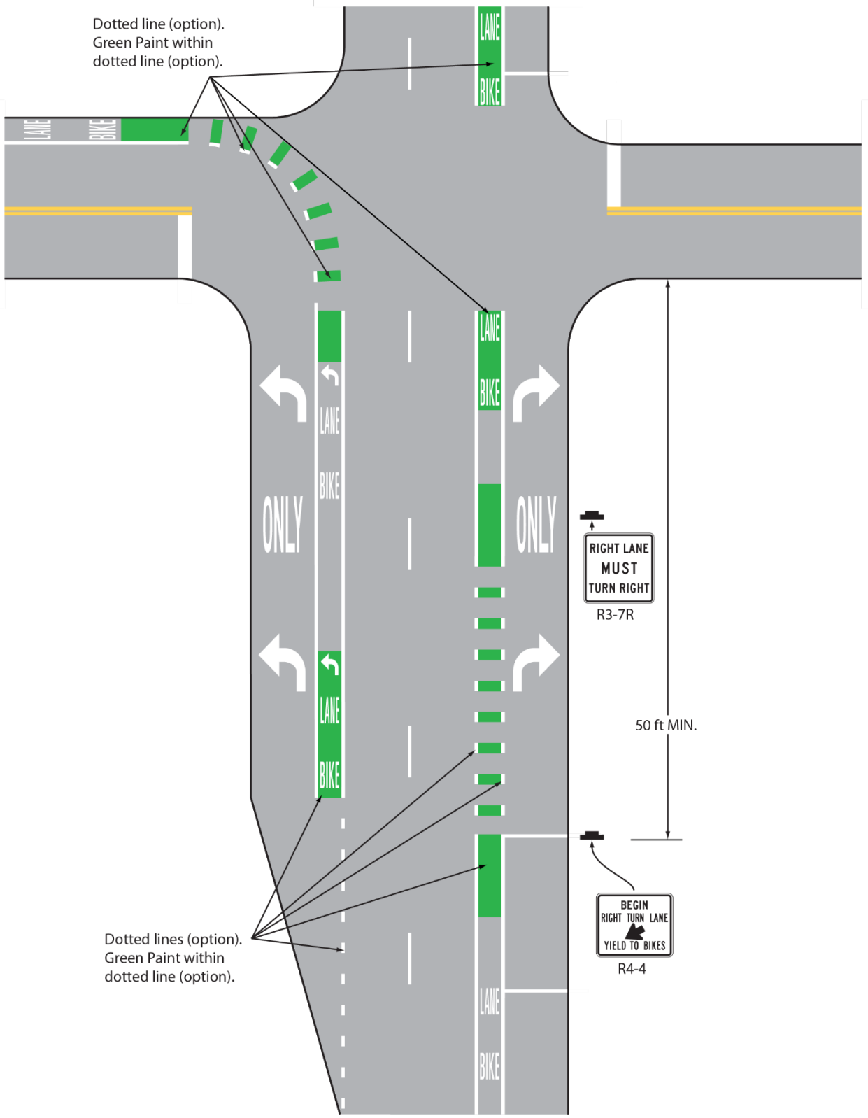
Figure 9C-1 (CA). Example of Intersection Pavement Markings – Designated Bicycle Lane with Left-Turn Area, Heavy Turn Volumes, Parking, One-Way Traffic, or Divided Highway
