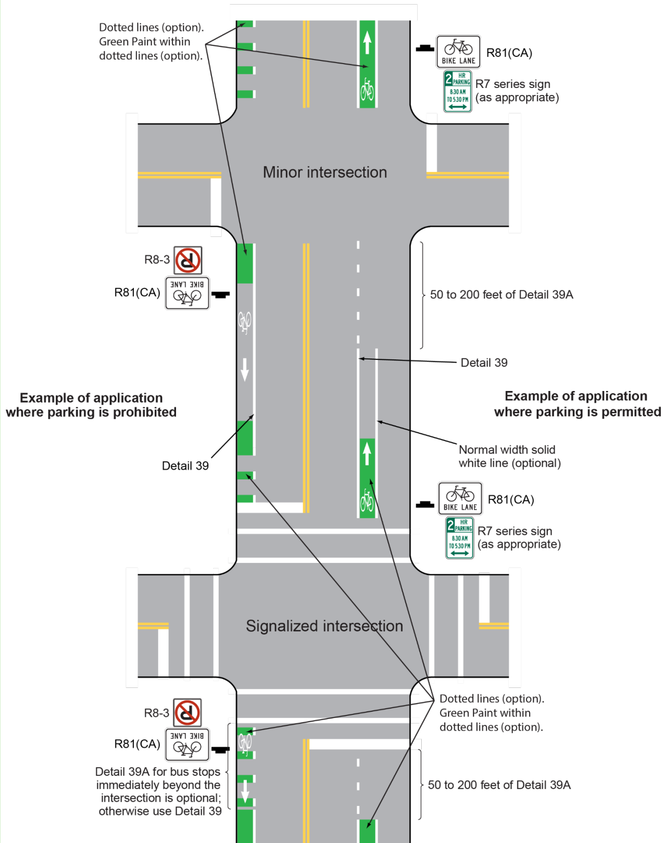
Figure 9C-6 (CA). Example of Pavement Markings for Bicycle Lanes on a Two-Way Street
