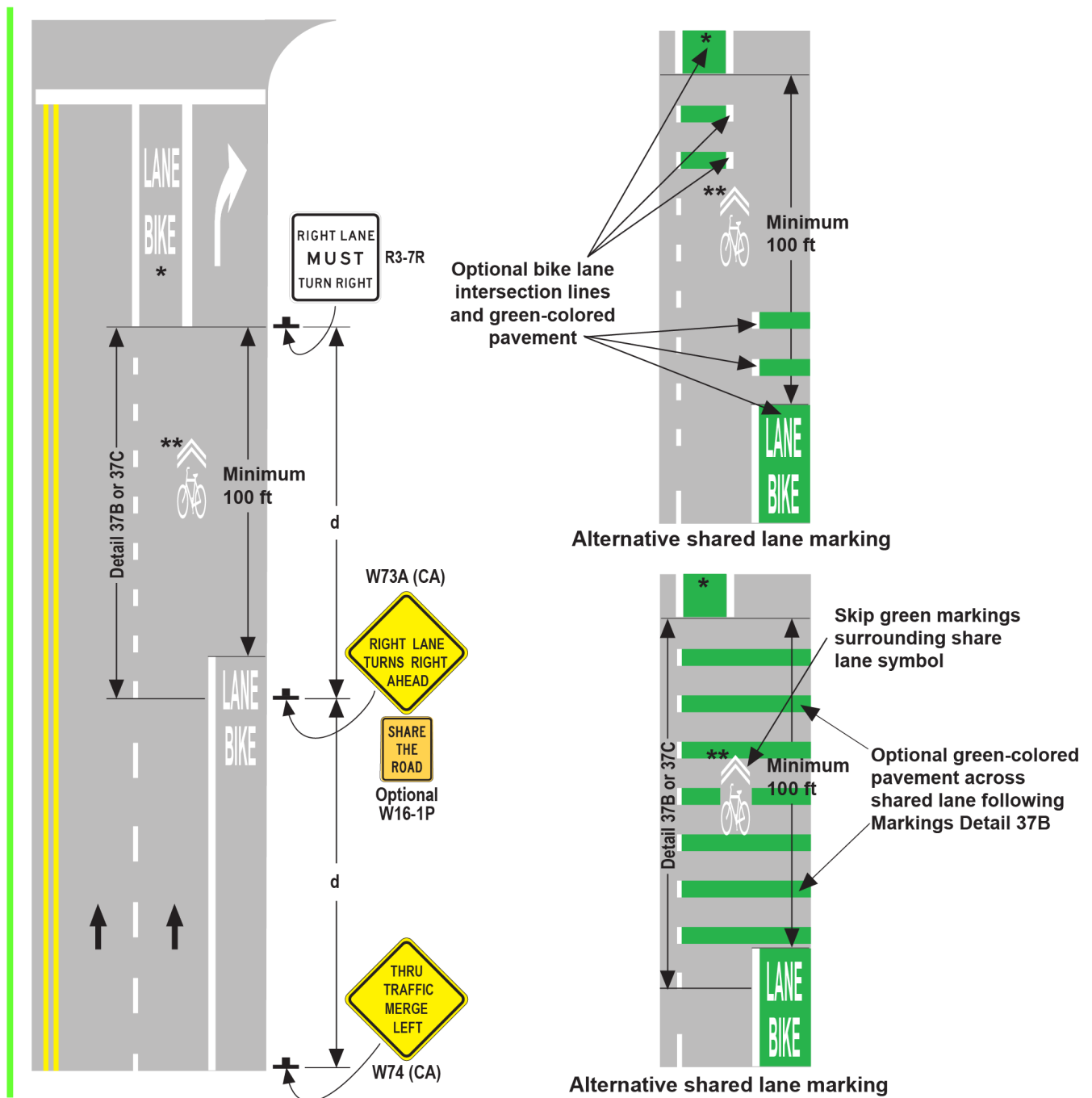
Figure 9C-109 (CA). Example of Shared Lane Marking While Approaching an Intersection
