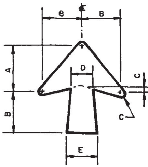
Arrow Detail
